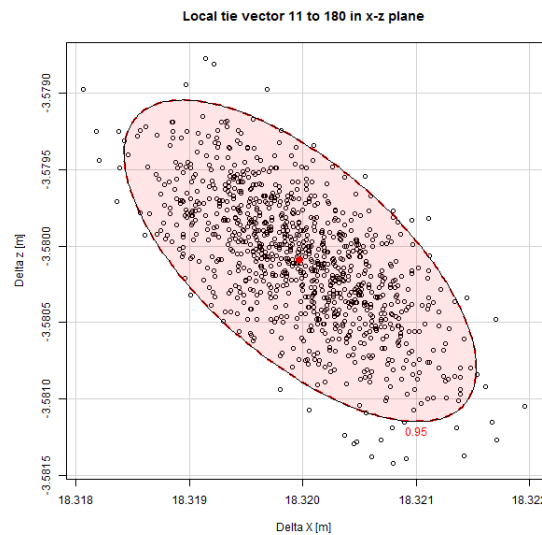
Figure 8 Local tie vector between points 11 and 180. The elliptical contours refer to a confidence level of 95%. The semi major axis is about 1.6 mm (x-y plane) and 2 mm (x-z plane)
