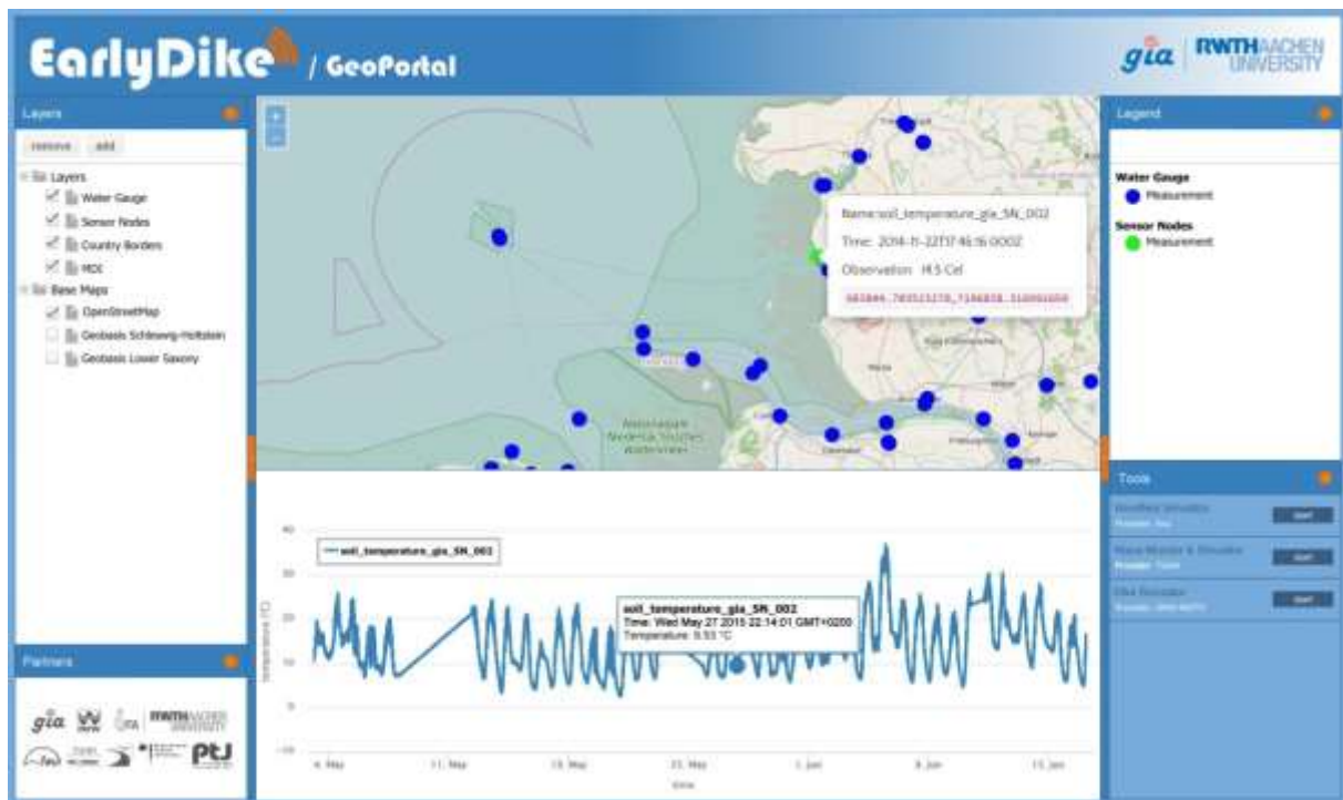
Fig. 6: EarlyDike GeoPortal
